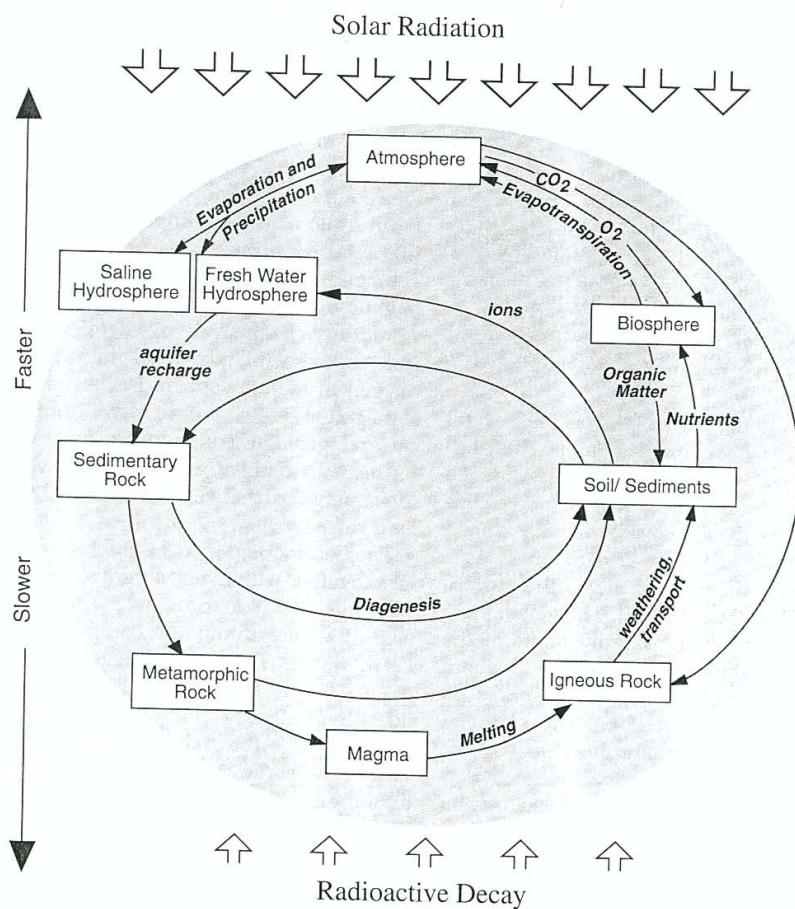
Fig. 1-1 Diagram of cyclic processes and fluxes between the major reservoirs on Earth.
