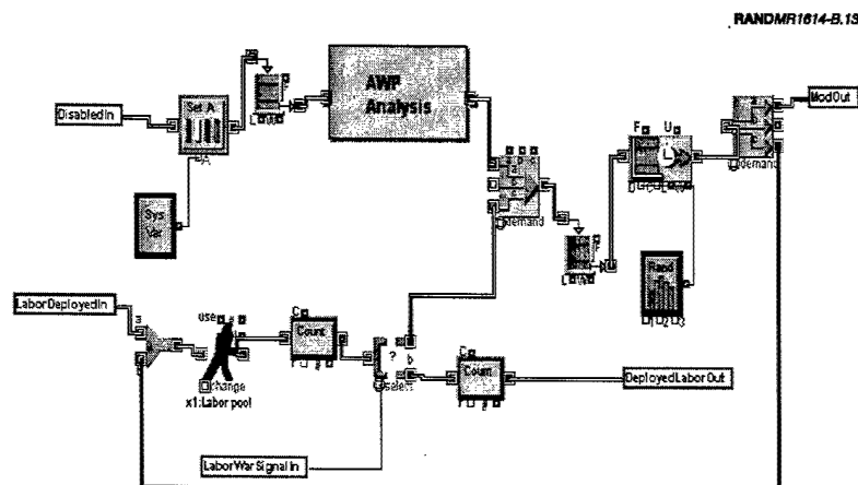
Figure B.13—JEIM Block at a Unit
