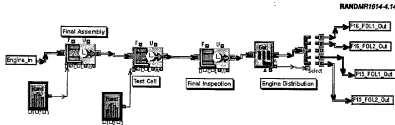
Figure 4.14—Assembly and Test Cell Block
