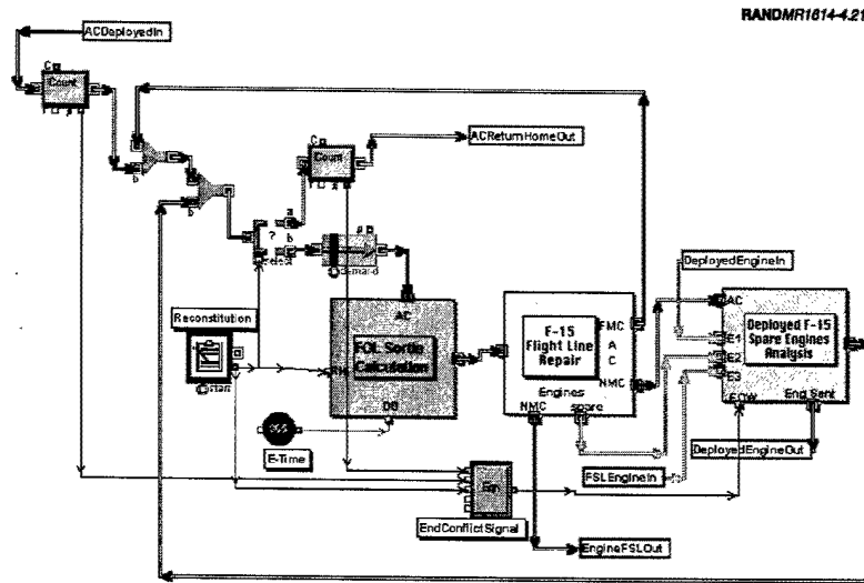
Figure 4.21—FOL Block
