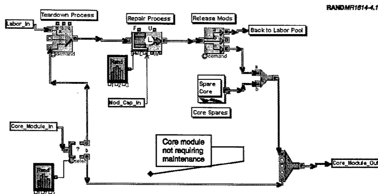
Figure 4.13—Core Module Repair Shop Block
