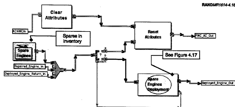
Figure 4.16—Spares Analysis Block at an F-15 Base
