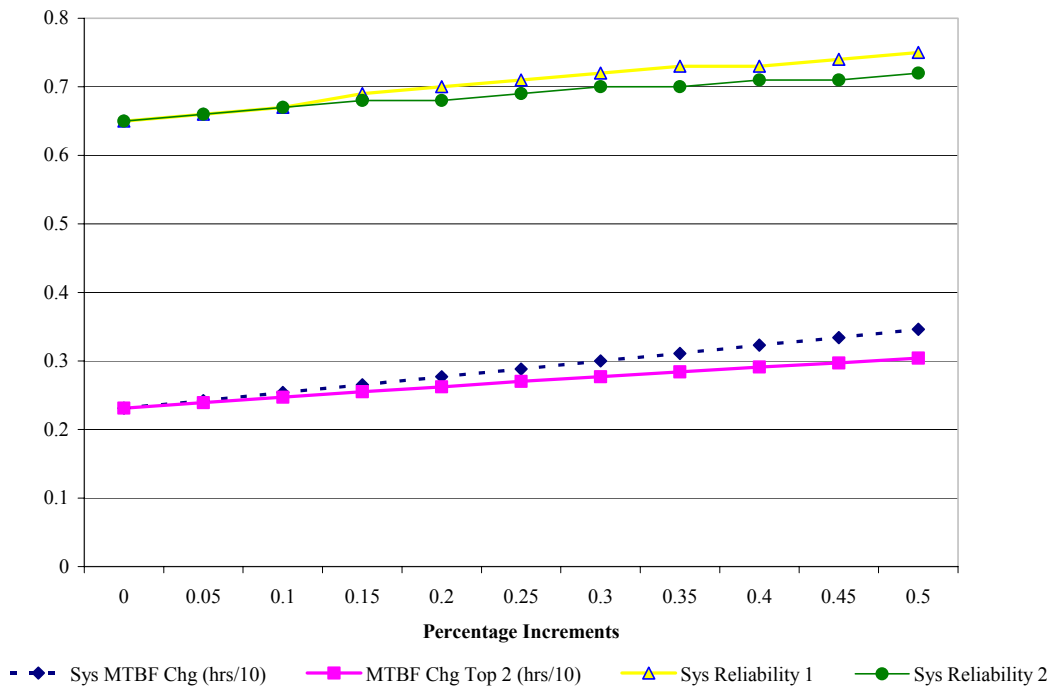
Figure 12. Comparison of Improvements in System Reliability versus Improvements in Reliability of Top Two Degraders.
