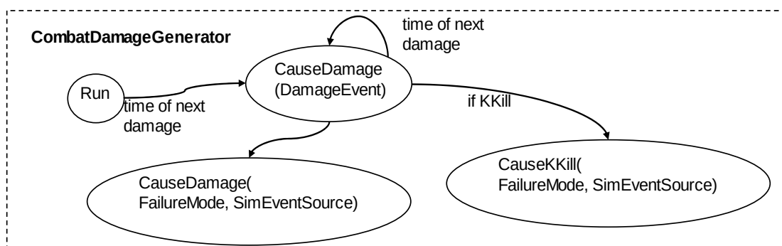
Figure 9. CombatDamageGenerator class
