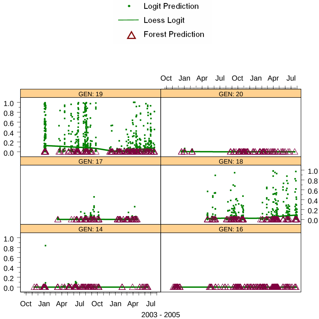
Plots of Estimated Probability of Bad from the Logistic Regression Model with Smoothing and the Classification of Being Good (0) or Bad (1) from the Forest of Trees Model for the Entire Two-Year Acquisition Period
