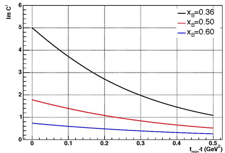
\Delta^2 -dependence of \Im m[C^I] in VGG model
