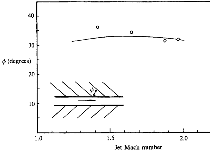
FIGURE 20. Comparison between calculated and observed angle of the wavefronts of the Kelvin-Helmholtz instability waves outside a supersonic helium jet. —, calculation (high frequency); \circ , experiment of Rosales (1970).
