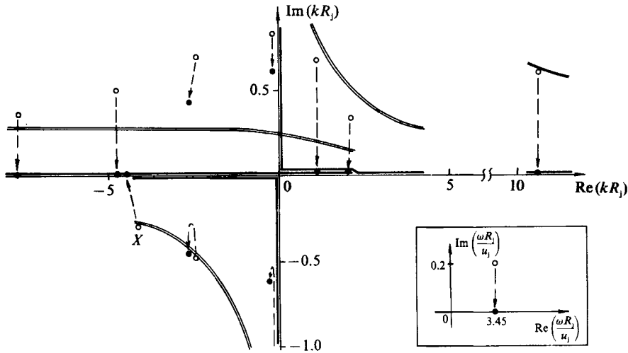
FIGURE 14. Trajectories of the zeros of D(\omega, k) in the complex k -plane as \text{Im}(\omega) \rightarrow 0^+ showing the upstream propagating subsonic wave marked by 'X'. Cold jet, Mach number 1.5, n = 0 .
