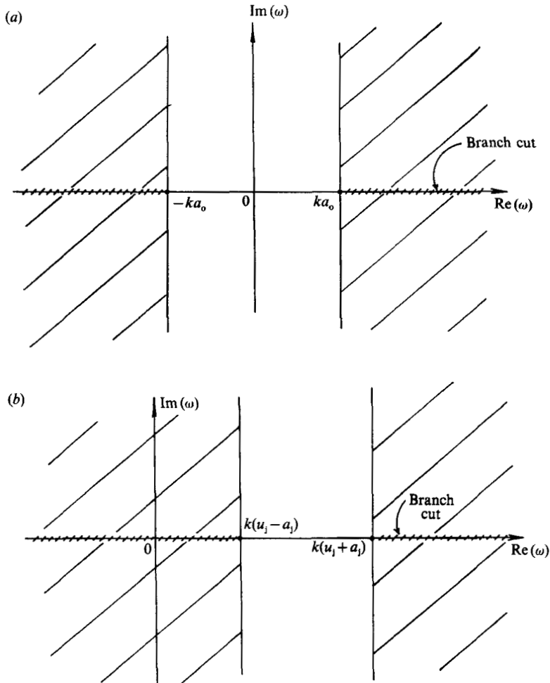
FIGURE 6. Branch cuts of (a) \eta_0 and (b) \eta_i in the complex \omega -plane for a supersonic jet. Shaded areas are regions with supersonic convective Mach number.
