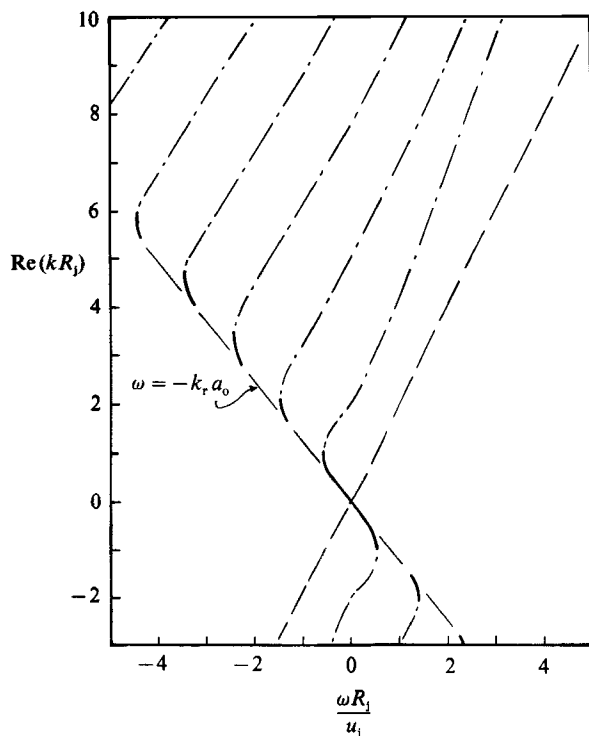
FIGURE 13. Dispersion relations, k_r(\omega) , of ---, the Kelvin-Helmholtz instability wave; — · — ·, the subsonic waves; —, and the upstream propagating subsonic waves. Cold jet, Mach number 1.5, n = 0 .
