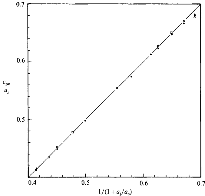
FIGURE 26. Correlation of the phase velocity of supersonic instability wave at maximum spatial growth rate with the parameter [1+a_j/a_0]^{-1} . \bullet , n=0 ; \times , n=1 ; \square , n=2 ( \gamma_j=\gamma_0 ).
