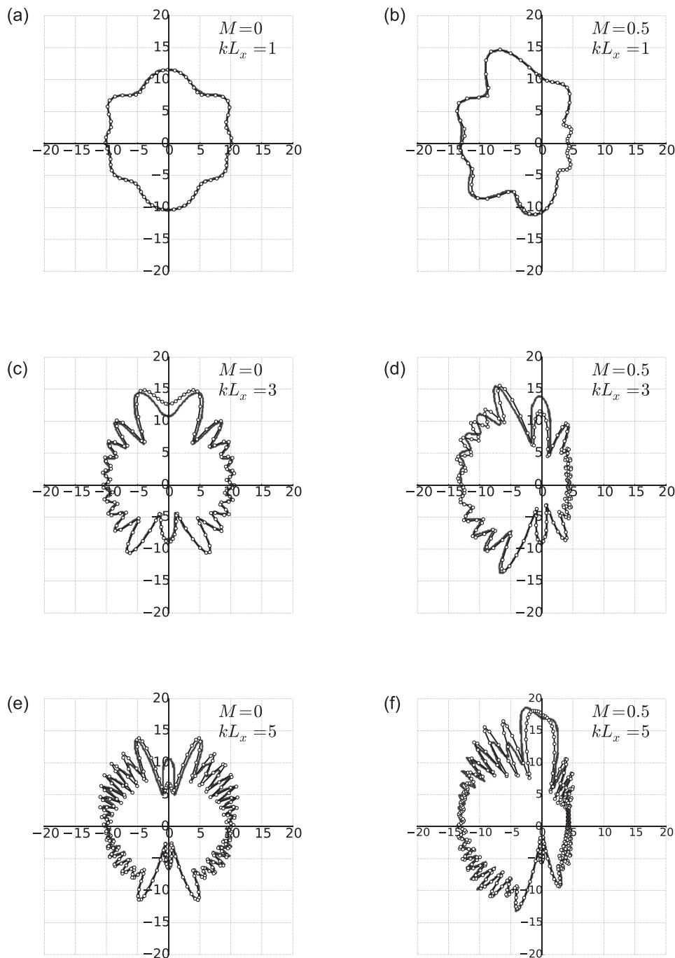
FIG. 4. Far field total pressure directivity patterns on the x - z plane, for the frequencies and Mach numbers as indicated. The horizontal and vertical directions represent, respectively, the x and z directions as defined in Fig. 3. Lines with symbols: Current calculation; Solid lines: Results from Ref. 3.
