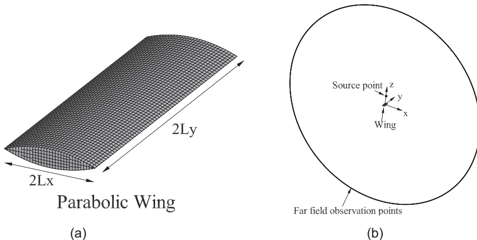
FIG. 3. A schematic of the computational setup. Left: dimensions of the parabolic wing and the surface mesh formed by 4364 quadrilateral elements, with L_x = 0.5 , L_y = 1.5 ; Right: a diagram of the scattering body, source point, and the far field observation point which is on the x - z plane and defined by \hat{\mathbf{r}} = (\hat{R} \cos \theta, 0, \hat{R} \sin \theta) and \hat{R} = 105L_x .
