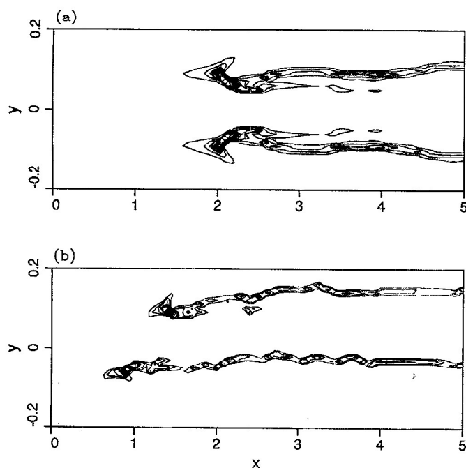
FIG. 5. Contours of the reaction rate. \Omega = \rho Y_F Y_O D e^{-Ze/T} with M=2 , u_j=2 , T_j=0.5 , Ze=20 , D=8 \times 10^7 , and \beta=2 . (a) \epsilon=0 , contour levels from 0.11 to 6.55, increment 0.11; (b) \epsilon=0.02 , k_2=4\pi , contour levels from 0.13 to 8.25, increment 0.13.
