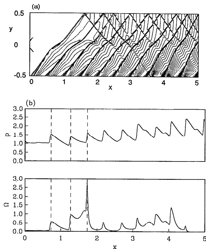
FIG. 4. (a) Contours of the pressure with M=2 , u_j=2 , T_j=1 , Ze=20 , D=4 \times 10^7 , \beta=2 , \epsilon=0.02 , and k_2=4\pi ; (b) pressure and reaction rate profiles versus x at y=-0.05 .
