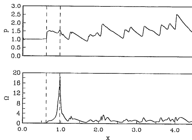
FIG. 6. Pressure and reaction rate profiles along the locus of maximum reaction rate for the lower reaction zone in Fig. 5(b). M=2 , u_j=2 , T_j=0.5 , Ze=20 , D=8 \times 10^7 , and \beta=2 .
