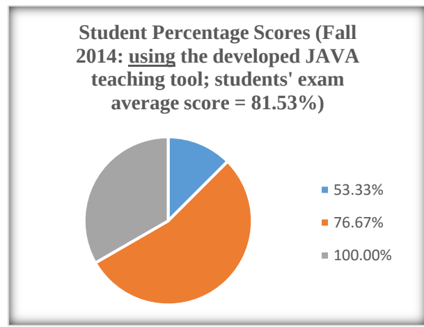
FIGURE 3 STUDENT PERCENTAGE SCORES (FALL 2014)
