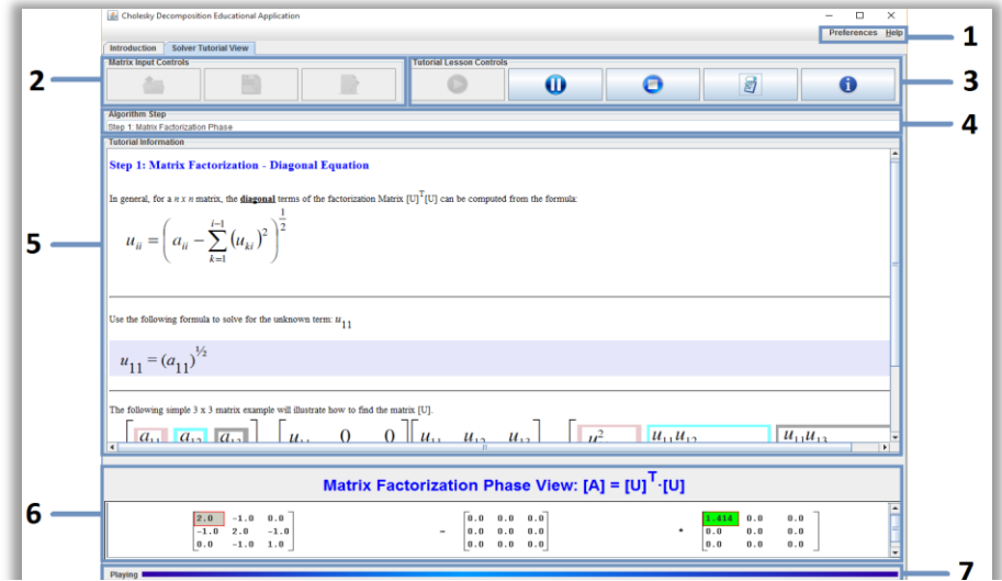
FIGURE 1 CHOLESKY DECOMPOSITION EDUCATIONAL APPLICATION
