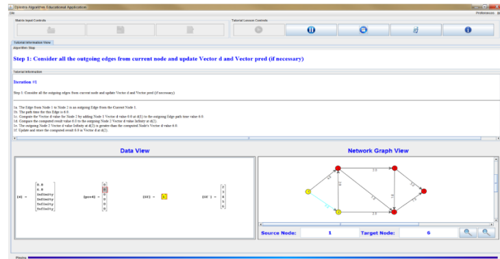
Figure 16: Main GUI (Step 1)
