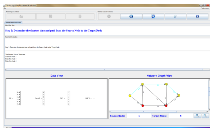
Figure 18: Main GUI (Step 3)
