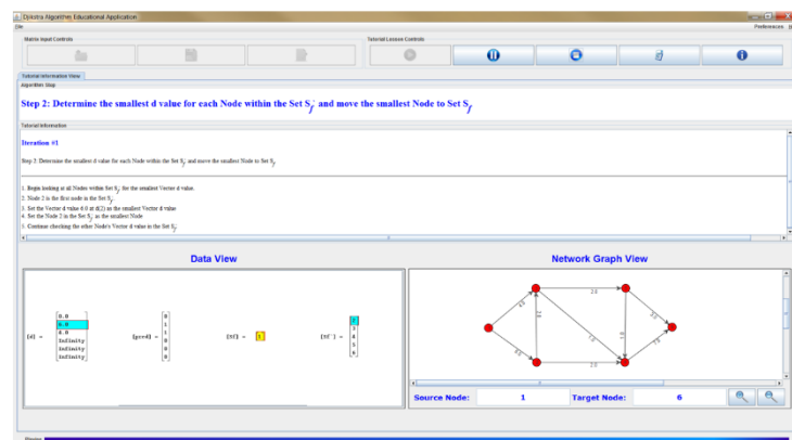
Figure 17: Main GUI (Step 2)
