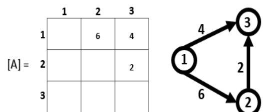
Figure 1: Matrix and Graph View of Nodes and Links
