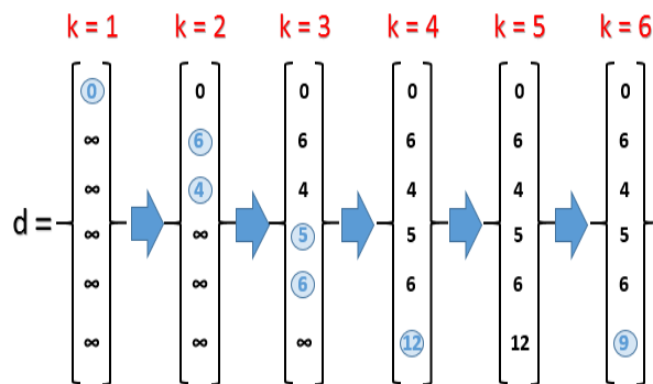
Figure 10: Vector [d] Updates During Iterations
