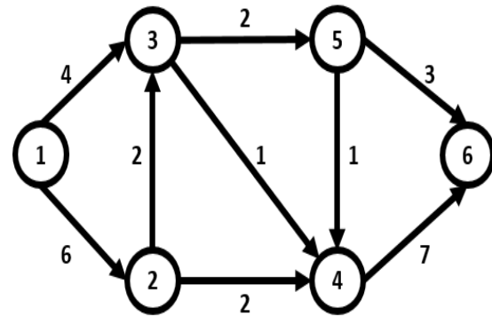
Figure 3: 6 x 6 Graph
