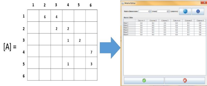
Figure 14: Matrix Editor (Matrix [A] Data)
