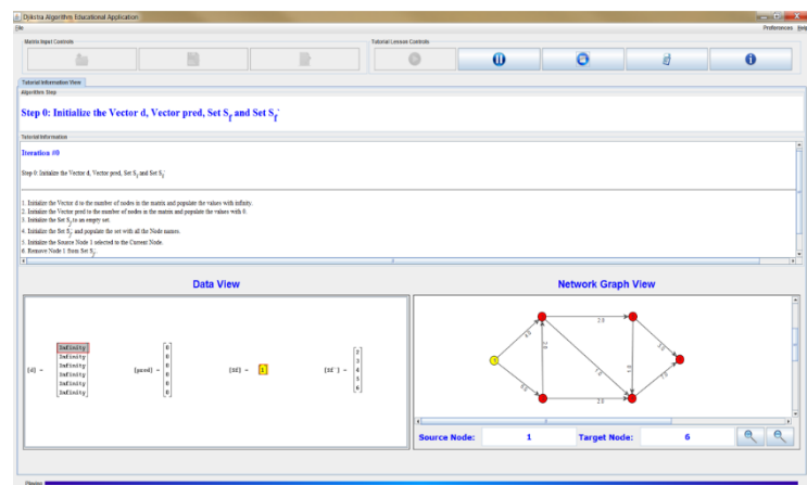
Figure 15: Main GUI (Step 0)
