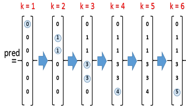
Figure 11: Vector [pred] Updates During Iterations
