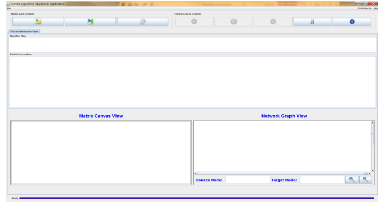
Figure 13: Main GUI
