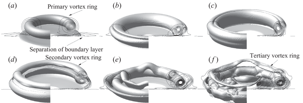
FIGURE 4. Evolution of vorticity iso-surface \|\boldsymbol{\Omega}\|=2.0 for the case of \theta=0^\circ and Re=830 . (a) T=5 , (b) T=7 , (c) T=8 , (d) T=9 , (e) T=11 , (f) T=15 .
