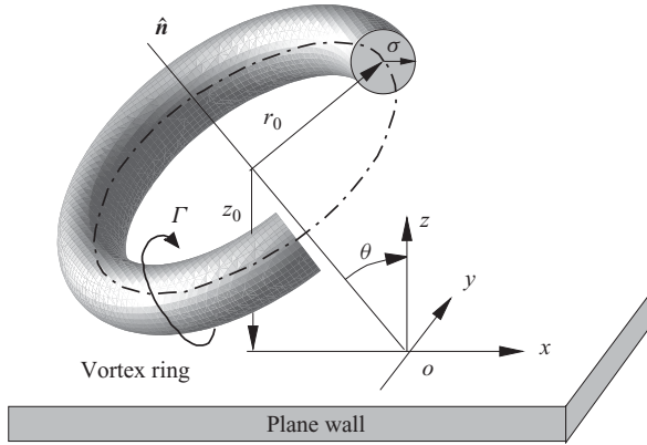
FIGURE 1. Schematic sketch of the geometry for a circular vortex ring approaching a plane wall.
