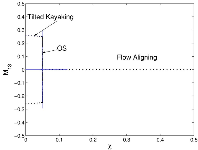
FIG. 3. M_{13} , time averaged, as a function of \chi at parameter values Pe=3.6 , \tilde{a}=0.8 and N=6 . In this parameter regime, the bistable attractors are tilted kayaking orbits in pure shear ( \chi=0 ). As \chi increases, the out-of-plane tilted kayaking orbits are arrested, leading to in-plane, steady distributions.
