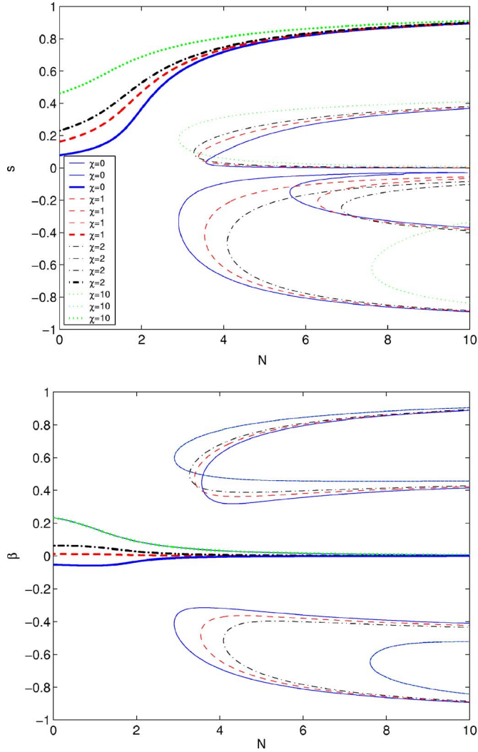
FIG. 6. The phase bifurcation diagram for planar extension flows subject to a transverse magnetic field with fixed weak extension rate Pe=0.1 , and variable (negative) magnetic anisotropy \chi=0, 1, 2, 10 , respectively. The thick curves depict stable solution branches of the model.
