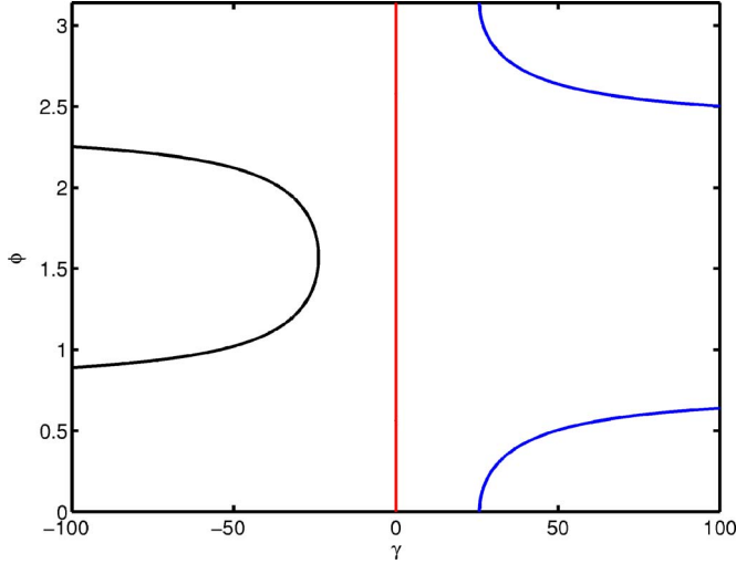
FIG. 4. The shear component \gamma in four-roll mill flows vs magnetic field angle \phi diagram for molecular aspect ratio r=3 ( a=0.8 ), which can be mapped to the reduced shear flow model with Pe=3.1 , \bar{a}=0.8 . G = Pe/2(1-\gamma) .
