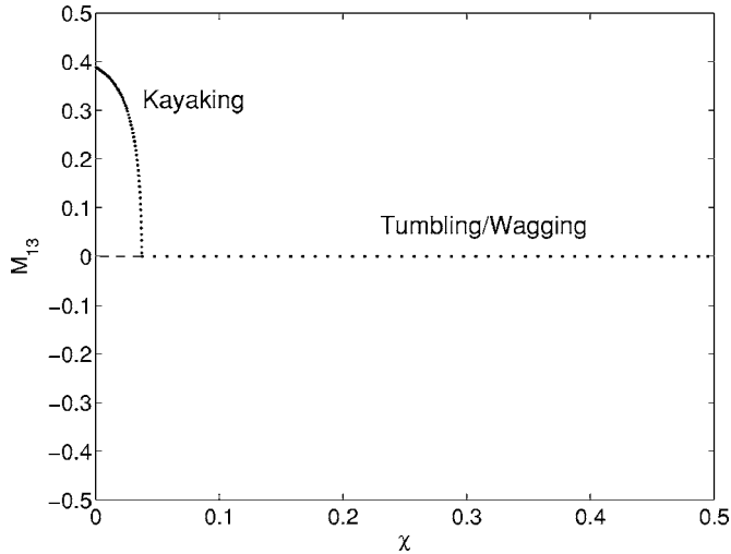
FIG. 1. Out-of-plane orientation tensor component M_{13} , time averaged, as a function of magnetic anisotropy \chi at parameter values Pe=1.5 , \bar{a}=0.8 and N=6 . As \chi increases, the out-of-plane kayaking orbit collapses onto an in-plane, tumbling orbit. The dotted curves indicate stability and all other curves correspond to unstable model solutions.
