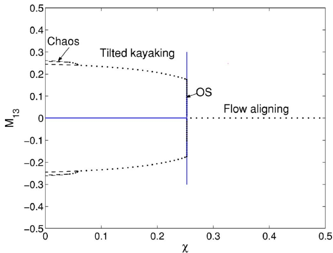
FIG. 2. M_{13} , time averaged, as a function of \chi at parameter values Pe=3.1 , \bar{a}=0.8 and N=6 . The shear response is chaotic for zero anisotropy \chi=0 . As \chi increases, the chaotic attractor spawns a pair of tilted kayaking orbits through a sequence of period-halving bifurcations, then at higher field strengths the limit cycle orbits are arrested, resulting in steady alignment. The dotted curves are stable solutions while the others are unstable model solutions.
