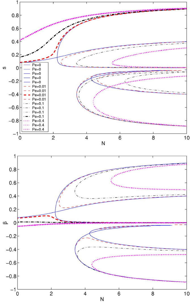
FIG. 7. The phase bifurcation diagram for planar extension flows subject to a transverse magnetic field with negative anisotropy \chi=1 , vs normalized extension rate Pe=0,0.01,0.1,0.4 , respectively. The thick curves depict stable solution branches.
