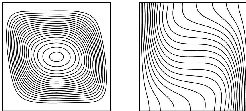
Figure 5: Streamlines and isotherms for Ra=10^4 in a cubical cavity ( y=0.5 ).
