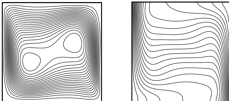
Figure 6: Streamlines and isotherms for Ra=10^5 in a cubical cavity ( y=0.5 ).
