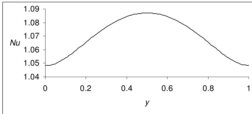
Figure 7: Distribution of the mean Nusselt number in the y -direction for Ra=10^3 .
