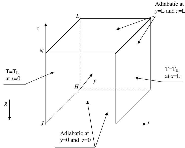
Figure 2: Configuration of the natural convection in a cubical cavity.
