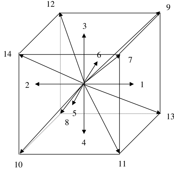
Figure 1: The lattice velocities of D3Q15.
