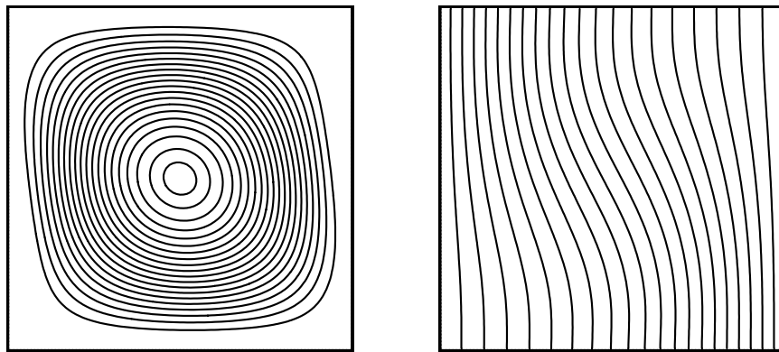
Figure 4: Streamlines and isotherms for Ra=10^3 in a cubical cavity ( y=0.5 ).
