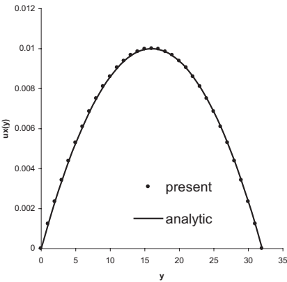
Fig. 2. Numerical velocity profile for the Poiseuille flow as compared with analytic solution.
