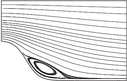
Fig. 10. Streamline for expansion channel flow at Re=10 .
