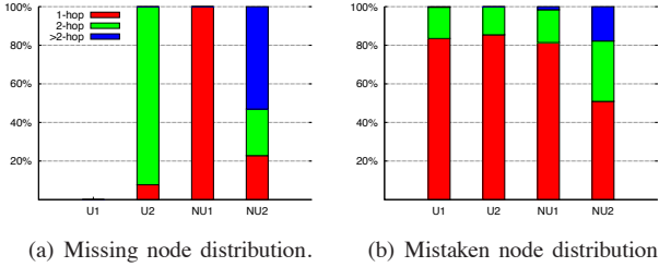
Fig. 2. Distributions of hop distances from missing and mistaken boundary nodes to nearest true boundary nodes. U1 and U2: Coconut and CABET under uniform sensor deployment, respectively; NU1 and NU2: Coconut and CABET under non-uniform settings.
